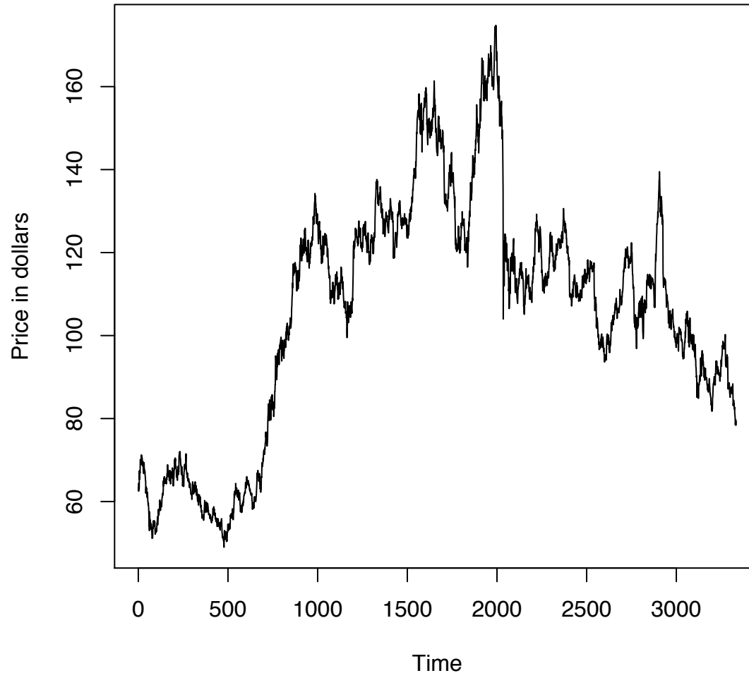
Daily closing price IBM: Jan 1, 1980–Oct 8, 1992
