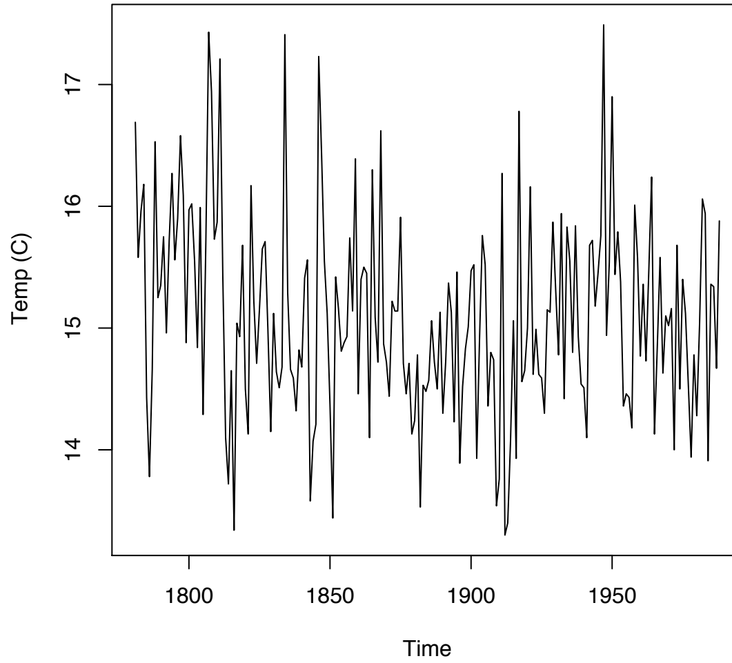
Mean Summer Temp: Munich, 1781–1988
