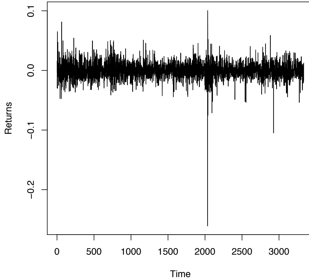
Daily returns IBM: Jan 1, 1980–Oct 8, 1992
