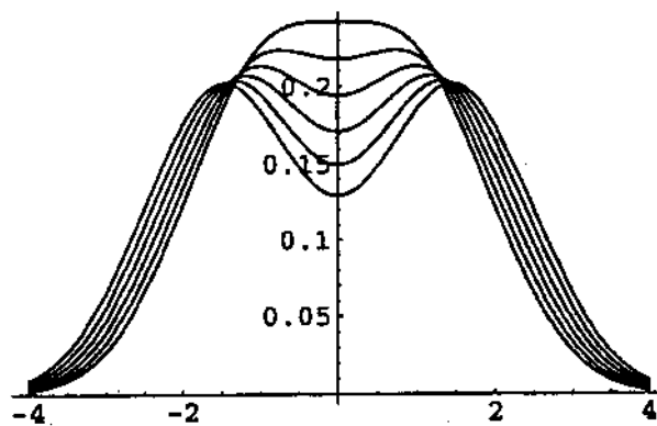
Figure 9. Six equal mixtures ( p = .5 ) of two normal densities. Each component has a standard deviation of 1. The values of |\mu_2 - \mu_1| are 2.0, 2.2, 2.4, 2.6, 2.8, and 3.0.
