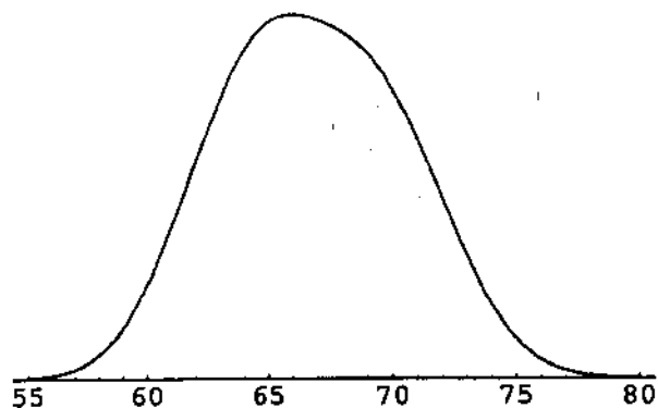
Figure 2. Theoretical distribution of U.S. young adult human height in inches as a mixture of two normal distributions using means and standard deviations from NHANES data.
