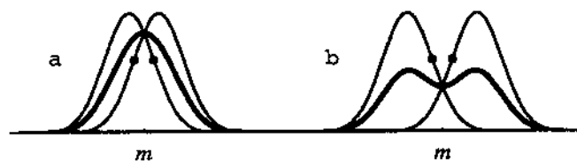
Figure 4. (a) When |\mu_1 - \mu_2| < 2\sigma , both normal components (light lines) are concave down at m = (\mu_1 + \mu_2)/2 , so the mixture f (heavy line) is also concave down at m and is therefore unimodal. (b) When |\mu_1 - \mu_2| > 2\sigma , both components are concave up at m , so the mixture f is also concave up at m , hence is bimodal. The dots indicate inflection points of the component densities.
